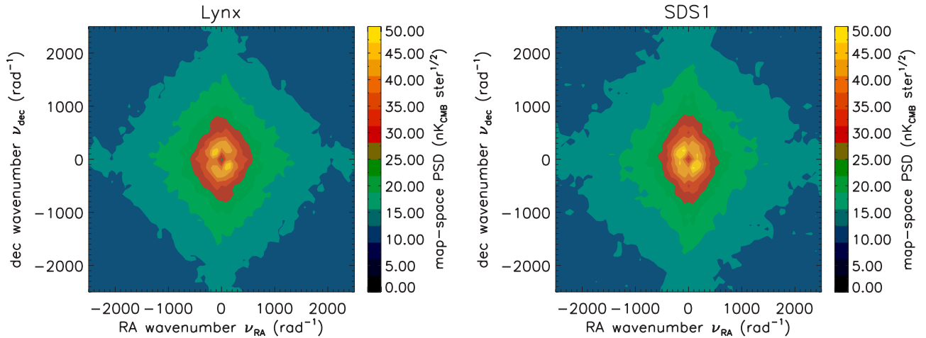
Figure 10. Map-space PSDs, P_v , of the maps made from co-adding all observations for a each science field. Note that relative to these PSDs, the power spectra of any astronomical signals will have been multiplied by the transfer functions of the data processing and the beam, T_v B_v^2 .
