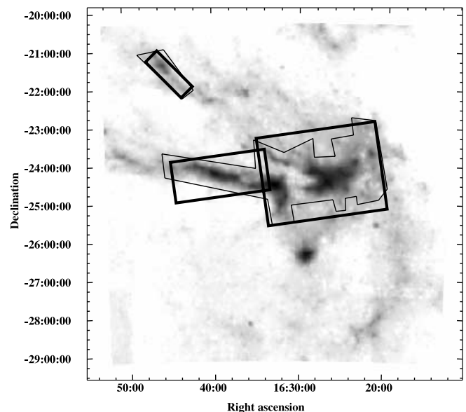
FIG. 1.—Extinction map of Ophiuchus from Cambr  s (1999), with the outline of the Bolocam observation area (thick lines) and the Spitzer IRAC observation area (thin lines). The area observed with IRAC was chosen to cover the cloud down to A_V \geq 3 . The Bolocam observations were designed to cover approximately the same region observed with IRAC.
