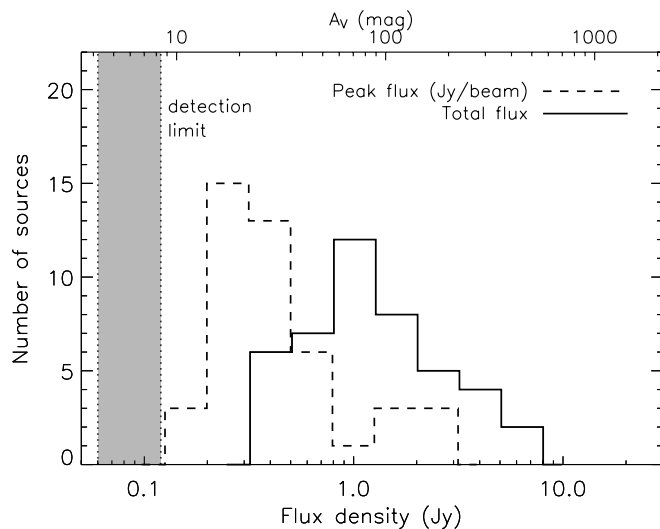
FIG. 7.—Distribution of the peak flux densities (dashed line) and total flux densities (solid line) of the 4\sigma sources. The peak flux density is the peak pixel value in the map, in \text{Jy beam}^{-1} . The top axis shows the value of A_V inferred from the emission, using eq. (2). The mean peak flux density of the sample is 0.6 \text{ Jy beam}^{-1} , and the mean total flux is 1.6 \text{ Jy} . The 4\sigma detection limit varies from 0.06 to 0.12 \text{ Jy beam}^{-1} across the map due to variations in the local noise, although most sources are detected in the higher noise regions. The range in noise is indicated by the shaded region.
