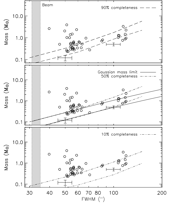
FIG. 11.—Distribution of source mass ( T_D = 10 K) vs. FWHM size. The size is the geometric average of the FWHM of the major and minor axes as given in Table 1. The maximum size of the pointing-smeared beam is represented by the shaded regions. Solid lines are the 50% analytic mass detection limit as a function of size for Gaussian sources (eq. [3]). Empirical 90% (top), 50% (middle), and 10% (bottom) completeness limits are indicated, derived using Monte Carlo methods with simulated sources and taking into account the effects of cleaning, iterative mapping, and optimal filtering. Each completeness limit is calculated both in a low rms region (bottom line) and a high rms region (top line). Most real sources are found in the higher rms regions. Representative error bars for 50'' and 100'' FWHM sources near the detection limit are shown, as estimated from the results of Monte Carlo simulations.
