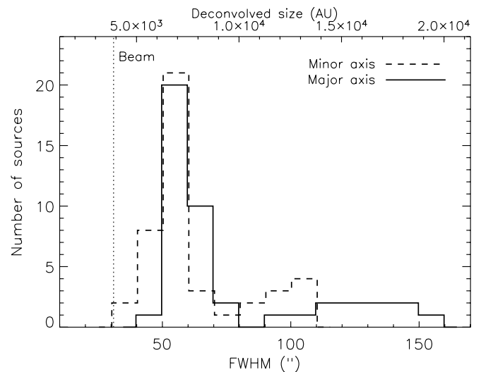
FIG. 8.—Distribution of source FWHM minor axis (dashed line) and major axis (solid line), as determined from an elliptical Gaussian fit. The beam size is indicated by the dotted line. The mean FWHM sizes of the sample are 62'' (minor) and 77'' (major). The top axis gives deconvolved sizes in AU, assuming a 31'' beam and d = 125 pc.
