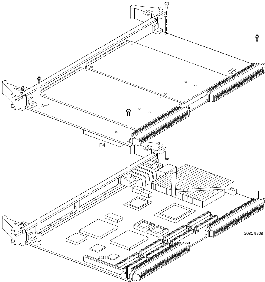
Figure 1-4. PMCspan-002 Installation on an MVME2300
