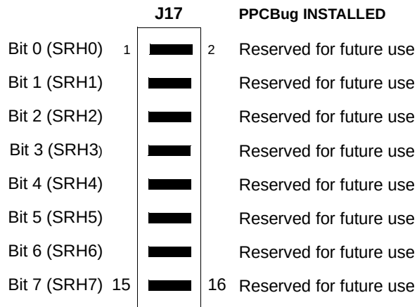
Figure 1-2. General-Purpose Software-Readable Header
