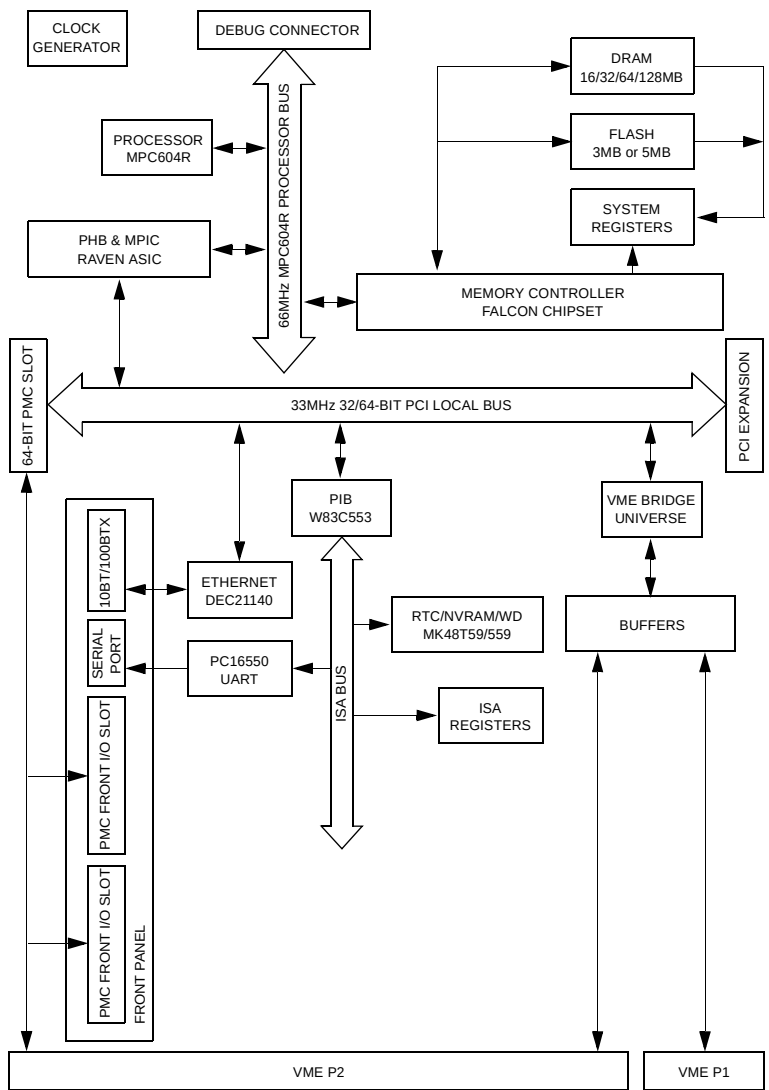
Figure 3-1. MVME2300 Block Diagram
