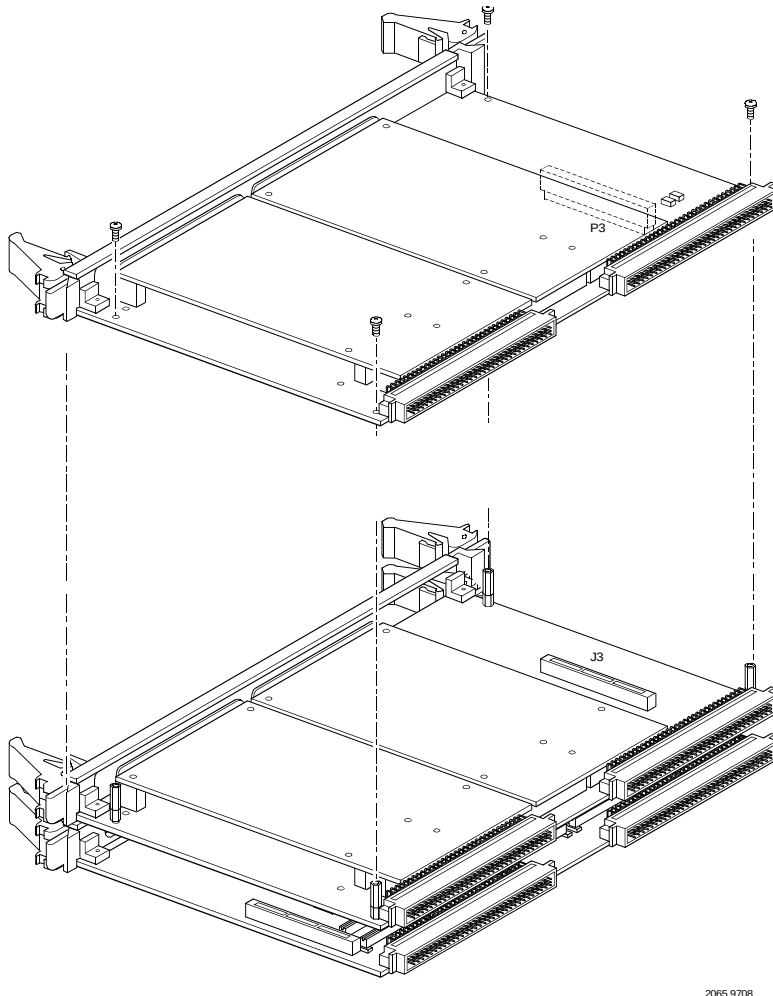
Figure 1-5. PMCspan-010 Installation onto a PMCspan-002/MVME2300
