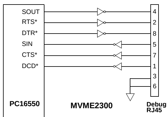
Figure 2-1. MVME2300 DEBUG Port Configuration
